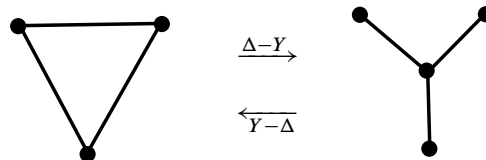
Figure 1: The Y\Delta and \Delta Y transforms.
