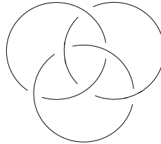
Figure 2: Borromean rings.
