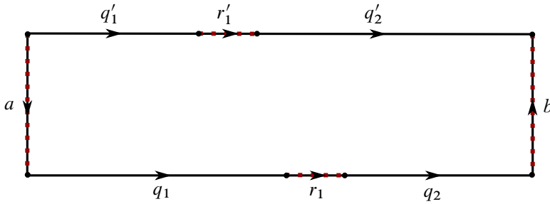
Figure 12: The geodesic octagon aq_1rq_2b(q'_1r'q'_2)^{-1} . Sides from the set B are given by the dotted paths.
