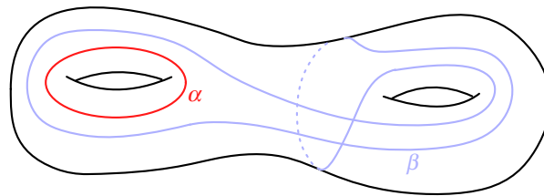
Figure 12: The two curves \alpha and \beta are homotopic through the handlebody pictured, and therefore bound an essential singular annulus. The only annuli one can produce from surgery are inessential, but one can surger to obtain the “obvious” disc in the picture that separates the handlebody into two solid tori.
