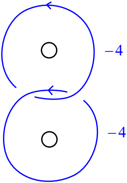
Figure 4: Surgery diagram of the branched double cover.
