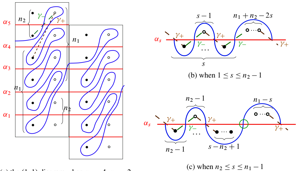
Figure 18: The case n_2 < n_1 . The only generators without a marking are given by the intersection point circled in (c).
