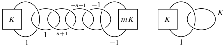
Figure 2: Left: an alternate surgery description of \mathrm{Sp}_{\phi_n^+}(K, mK) , obtained by blowing up two clasps in Figure 1. This identifies \mathrm{Sp}_{\phi_n^+}(K, mK) with \mathrm{Sp}_{\phi_{n+1}^+}(K', mK') where K' \subseteq Y' = Y_{+1}(K) is the dual knot of K . Right: the knot K' \subseteq Y_{+1}(K) .
