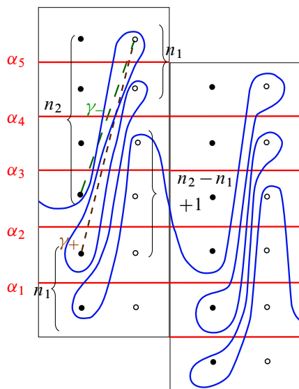
(a) the (1, 1) diagram when n_1 = 2, n_2 = 4
