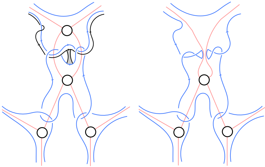
Figure 8: Handle slides in MK1.
