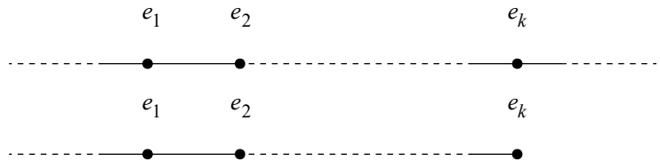
Figure 12: A chain in a plumbing graph [17].
