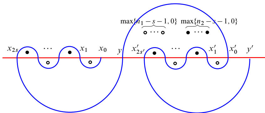
Figure 13: Two consecutive blocks H(s) (on the left) and H(s+1) (on the right) in G(s) for 1 \leq s \leq \min\{n_1, n_2, \lfloor \frac{n_1+n_2-1}{2} \rfloor\} . There could be other basepoints (at most more of each kind) in H(s+1) in the lower half plane.
