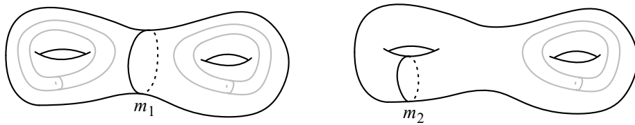
Figure 1: Compression bodies inside a genus-2 handlebody.
