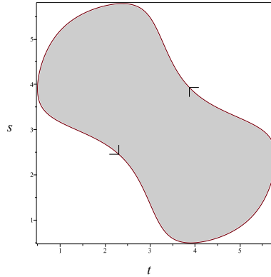
Figure 4. The Deninger chain \Gamma corresponding to (5-6).
