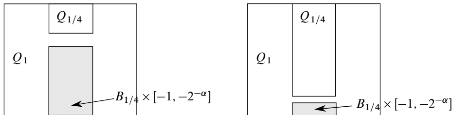
Figure 2. The cylinders Q_{1/4} and B_{1/4} \times [-1, -2^{-\alpha}] with large \alpha (left) and small \alpha (right).
