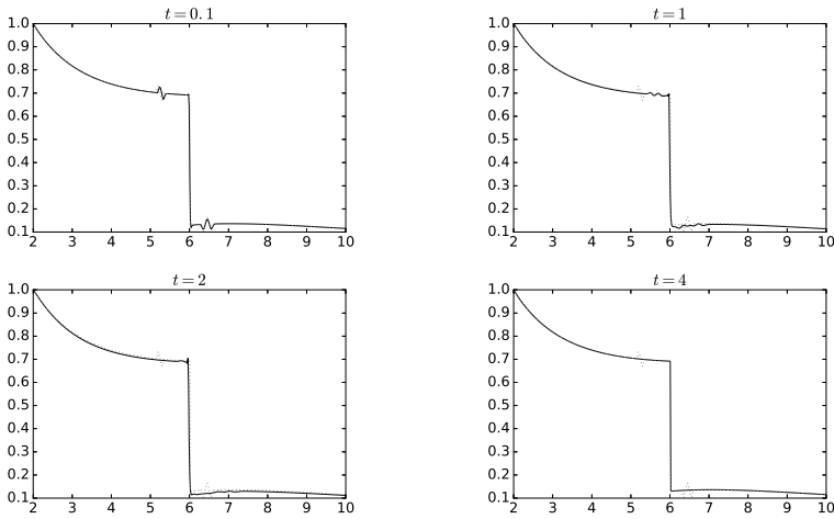
Figure 21. Euler: evolution of a perturbed steady state shock — convergence to the same steady state.
