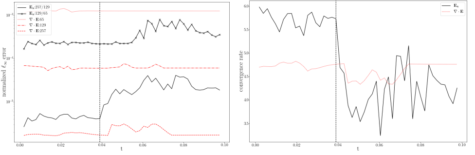
Figure 4. \ell_\infty error values and convergence results for E_x and \nabla \cdot E - 4\pi\rho for the stopped spherical charge distribution problem as a function of time in \Omega_2 . On the left are the normalized \ell_\infty errors for E_x and \nabla \cdot E - 4\pi\rho . The errors for E_x are obtained from the difference of sampled field values from N = 257 with N = 129 and also from sampled N = 129 with N = 65 test case. The E_x error is normalized by the max norm of the electrostatic solution ( \approx 0.0694795 ) and \nabla \cdot E - 4\pi\rho error is normalized by \max_{\mathbf{x}} 4\pi\rho \approx 30.6796 . On the right are the associated convergence rates. The vertical line indicates the time at which the charge distribution stops moving.
