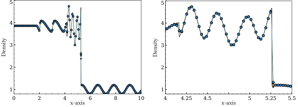
Figure 16. Shu–Osher test case: profile of density with PPM and WENO methods for N_x = 1024 . Left: full domain. Right: zoom.
