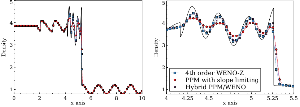
Figure 2. Shu–Osher test case: profile of density for N_x = 256 . Left: full domain. Right: zoom.
