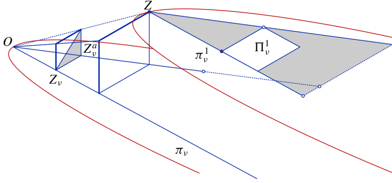
Figure 1. The central projection \mathfrak{P} .
