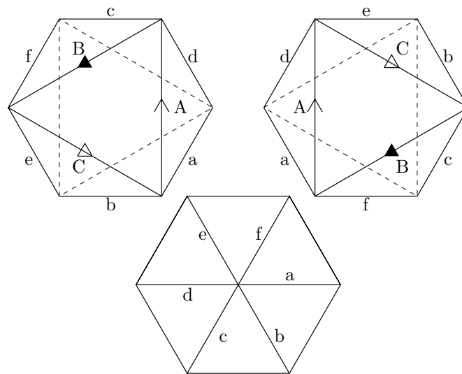
Figure 6: How to glue up the manifold
