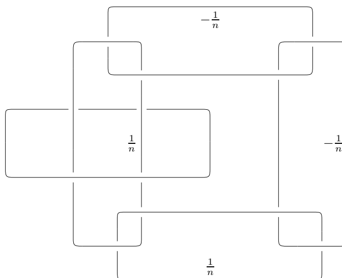
Figure 7: Knots with meridian length \rightarrow 4 as |n| \rightarrow \infty
