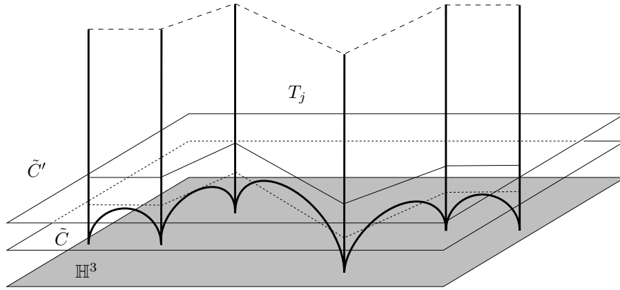
Figure 1: Shrinking the horocusp
