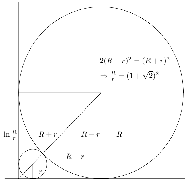
Figure 4: Bounding translation length
