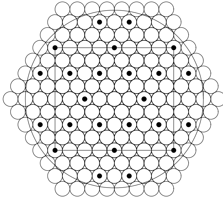
Figure 8: Primitive lattice points in the figure eight knot sister
