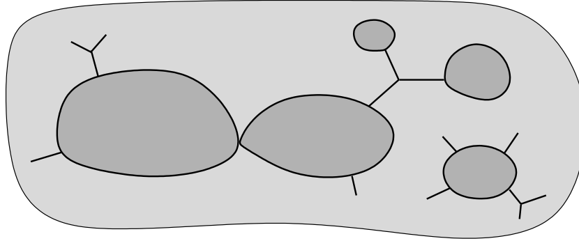
Figure 14: A reduced disc diagram \phi: D \rightarrow X and the preimage under \phi of some flat plane F in X . The preimage shown is disconnected and contains exactly five preflats.
