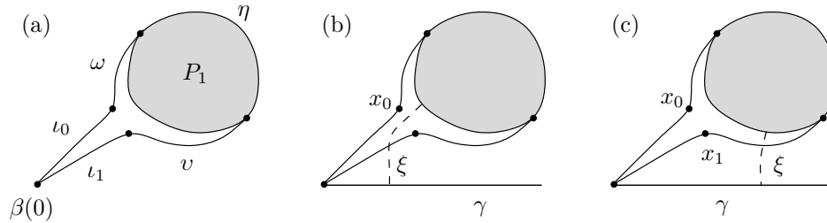
Figure 27: (a) The convex hull of the preflat P_1 and the point \beta(0) (b) The path \xi intersects \iota_1 . (c) The path \xi intersects \eta v .
