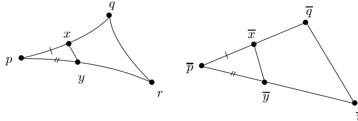
Figure 3: A comparison triangle and a pair of comparison points for the CAT(0) inequality
