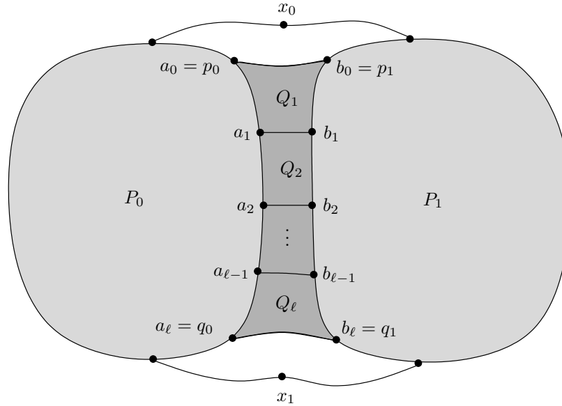
Figure 23: The preflats P_0 and P_1 map to the same flat in X . The darkened diagram is a geodesic quadrilateral Q with corners p_0, p_1, q_0, and q_1 . This quadrilateral has been subdivided into \ell smaller quadrilaterals Q_k .
