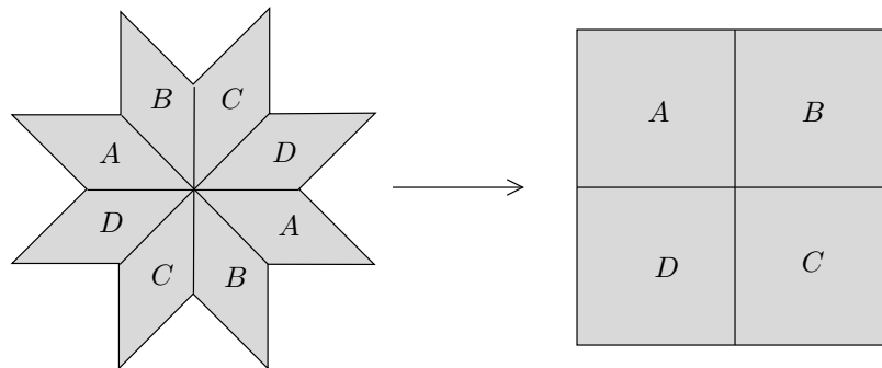
Figure 6: A reduced map from a disc diagram to a nonpositively curved squared 2-complex. The diagram on the left inherits a CAT(0) metric in which the eight 2-cells are Euclidean squares.
