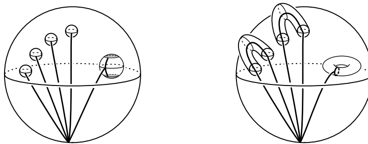
Figure 2: The graph G_{n,k} in M_{n,k}
