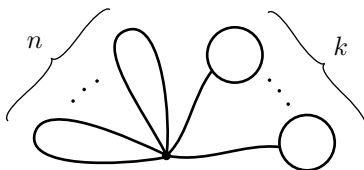
Figure 1: The graph G_{n,k}
