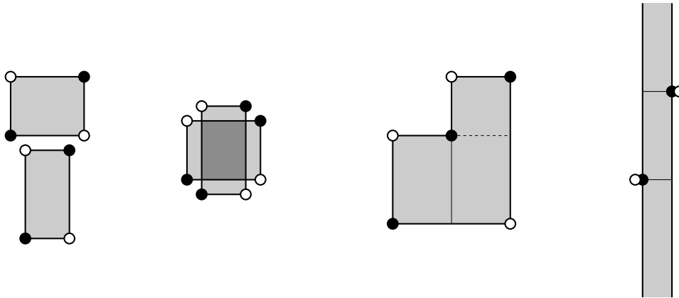
Figure 3: \partial^- \circ \partial^- = 0 . The four combinatorially different ways the composite of two empty rectangles r_1 * r_2 can appear. The initial point is indicated by the dark circles, the final by the hollow ones.
