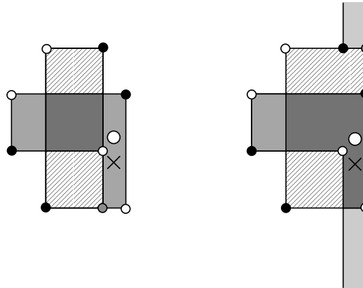
Figure 15: Cases I(1') and II(1). There are two terms in \partial \circ F^L + F^L \circ \partial starting at the black dots and ending at the white dots, thought of as elements of \mathcal{L} . The term on the left is a juxtaposition r * p (as in I(1')), while the second is p' * r' , where p' is of type L and r' is of Type 2 (as in II(1)).
