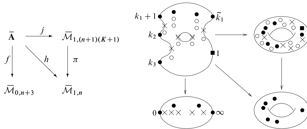
Figure 2: Four moduli spaces
