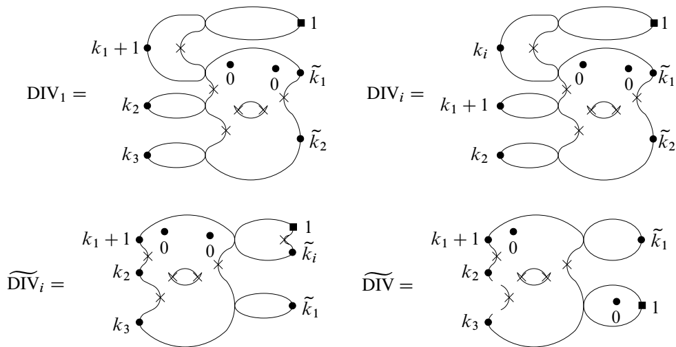
Figure 3: Divisors in \overline{\mathbf{A}}
