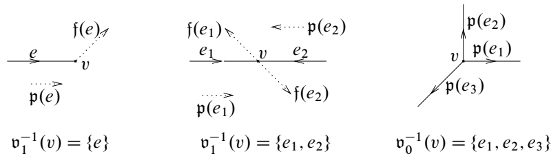
Figure 3: The position map p and the framing map f
