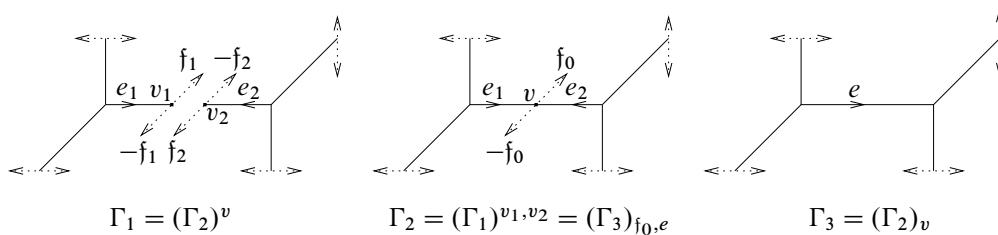
Figure 5: Operations on FTCY graphs
