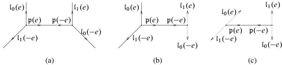
Figure 4: l_0, l_1: E^\circ(\Gamma) \rightarrow \mathbb{Z}^{\oplus 2} . (a) v_0(e), v_1(e) \in V_3(\Gamma) (b) v_0(e) \in V_3(\Gamma), v_1(e) \in V_1(\Gamma) \cup V_2(\Gamma) (c) v_0(e), v_1(e) \in V_1(\Gamma) \cup V_2(\Gamma)
