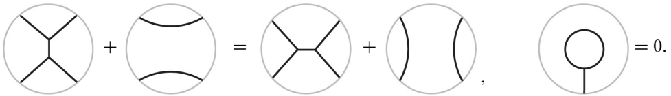
Figure 4: Relations in the trivalent presentation of the chromatic algebra
