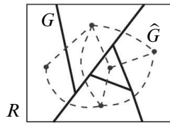
Figure 3: A basis element G of the algebra \mathcal{F}_2 and the dual graph \hat{G} (drawn dashed)
