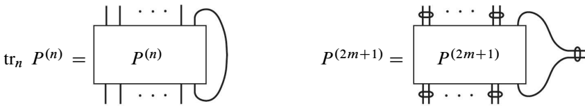
Figure 29: The identity on the right holds in the Temperley–Lieb category at d = 2 \cos(\pi j / (2m + 2)) .
