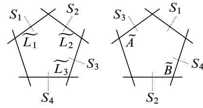
(b) Configuration of sections
