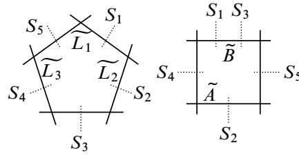
(b) Configuration of sections
