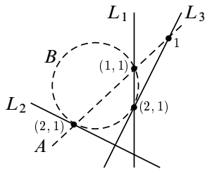
(a) The pencil of cubics. L_1 + L_2 + L_3 : three lines A + B : line+conic
