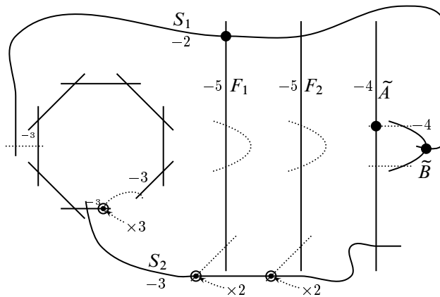
Figure 12: A rational surface Z'' = Y \# 8\bar{\mathbb{P}}^2
