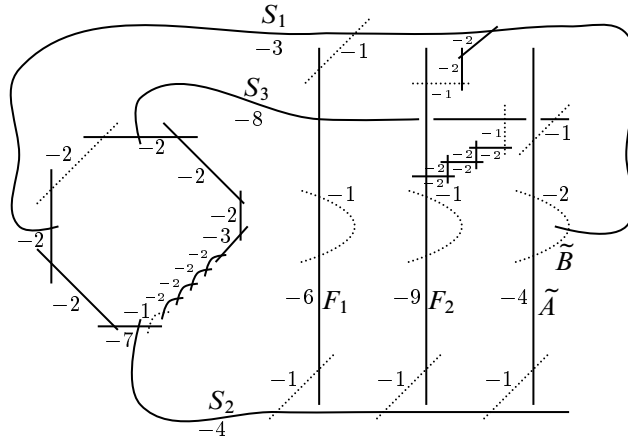
Figure 5: A rational surface Z = Y \# 21\overline{\mathbb{P}}^2
