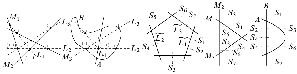
(a) The pencil of cubics. L_1 + L_2 + L_3 : three lines M_1 + M_2 + M_3 : three lines A + B : line+conic
