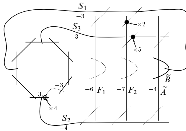
Figure 4: A rational surface Z'' = Y \# 10\mathbb{P}^2
