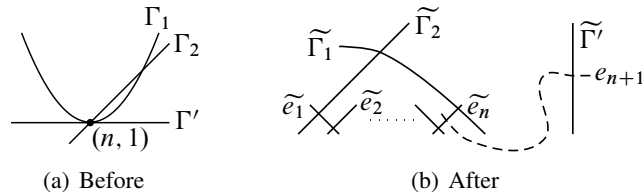
Figure 6: Blowing up at nodes
