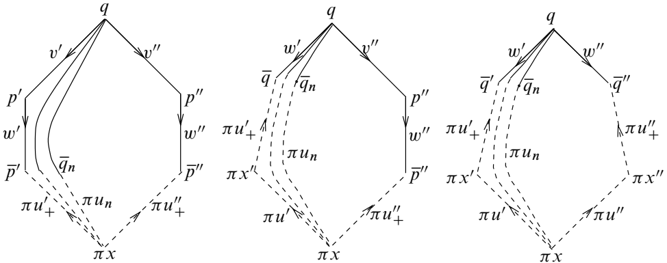
Figure 3: Solid lines are -\nabla\mathcal{E} trajectories in N and dotted lines are the projections under \pi: T^*N \rightarrow N of Floer solutions.
