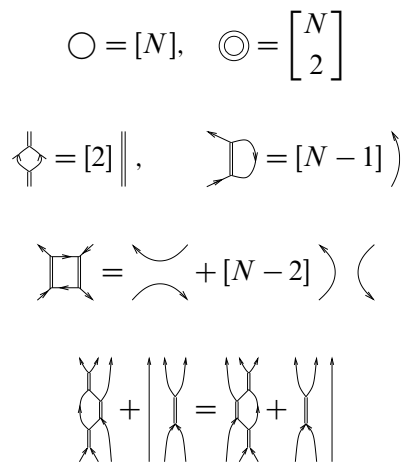
Figure 3: MOY web moves
