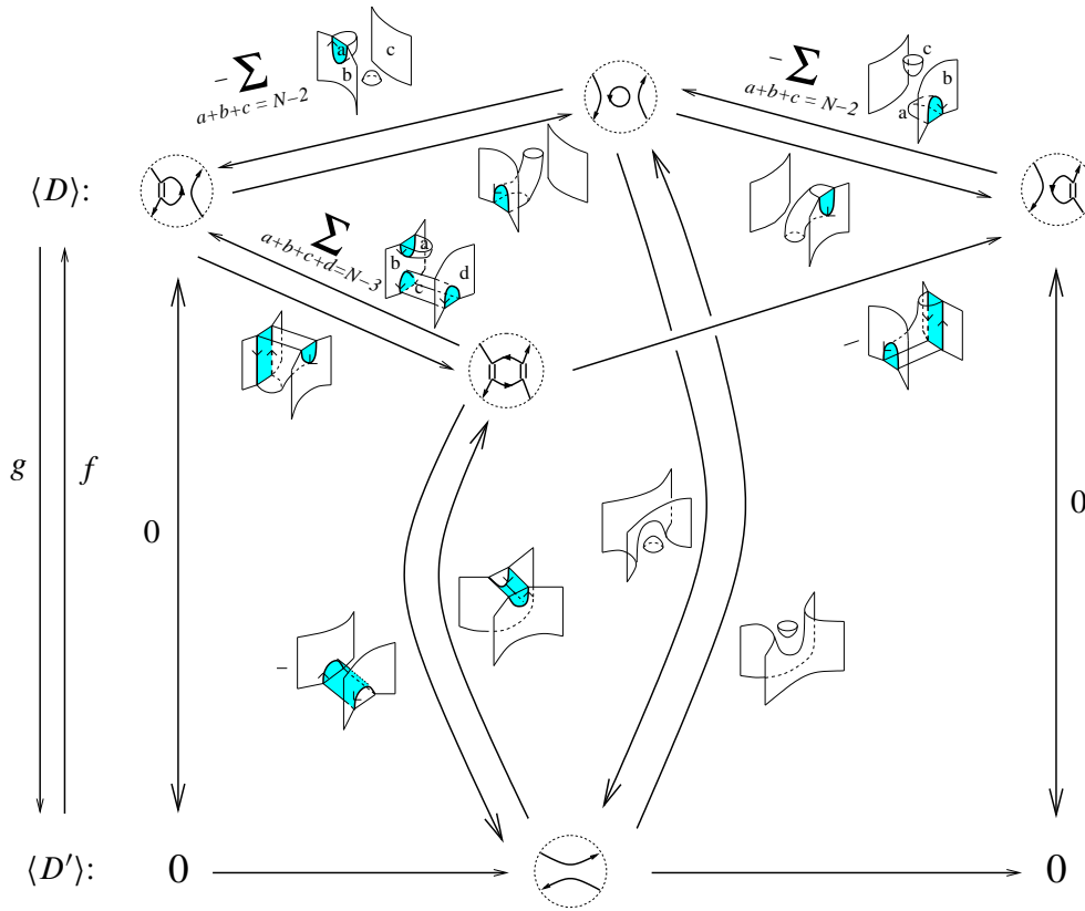
Figure 10: Invariance under Reidemeister IIb
