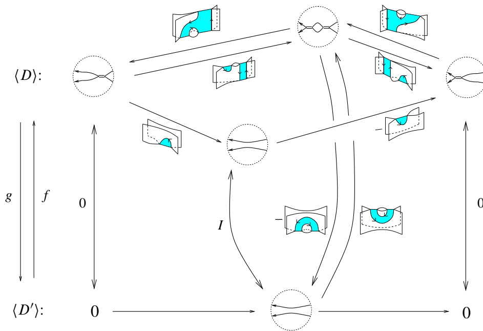
Figure 9: Invariance under Reidemeister IIa
