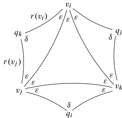
Figure 7: Generalized circle packing
