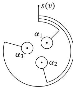
Figure 1: The canonical basis
