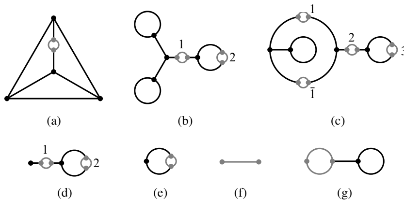
Figure 5: The skeletons Sk' and Sk
