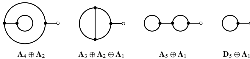
Figure 11: Perturbations of E_7 with nonabelian fundamental group
