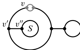
Figure 8: The set of singularities E_7 \oplus 2A_6
