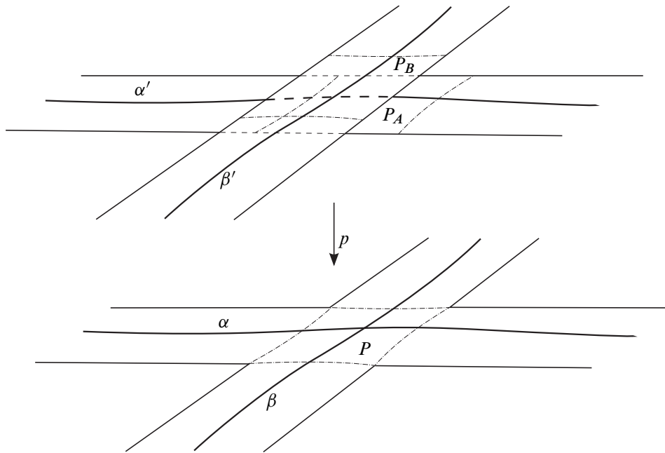
Figure 1: The quasipolygon P in the lower sutured diagram defines a decomposing surface S . The upper sutured diagram corresponds to the manifold obtained by decomposing along S .
