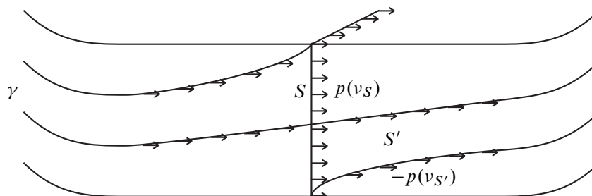
Figure 2: The decomposing surfaces S and S'
