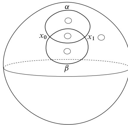
Figure 4: A sutured diagram for T(1, 0; 4)
