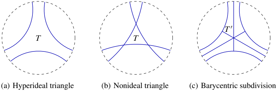
Figure 2: Hyperbolic triangles
