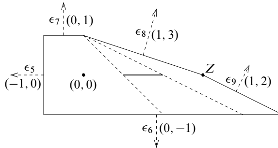
Figure 1: The polygon \tilde{\Delta} . The heavy line segment in the middle are the points that are nondisplaceable by probes. The conormals of \tilde{\Delta} are the vectors v_5, \dots, v_9 in Equation (2-2) with \kappa = (1, 1, 1, 3, 3) .
