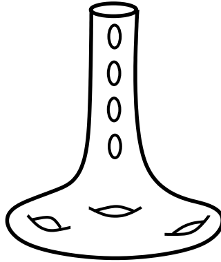
Figure 1: Surface with T_\infty -end
