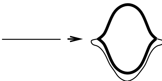
Figure 20: The embedding g
