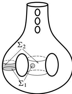
Figure 2: \Sigma_1 \subset \Sigma_2 \subset F
