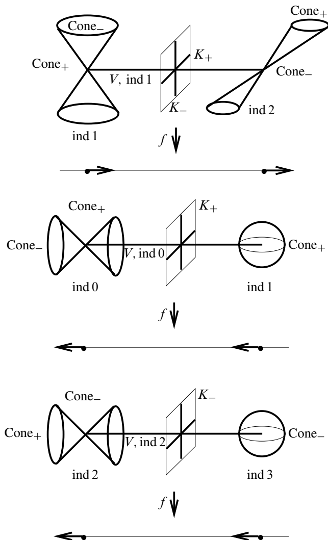
Figure 7: Mixed membranes ( n = 1, d = 2 )
