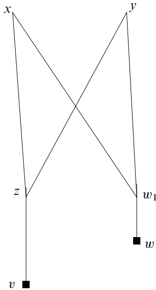
Figure 1: The loop in the proof of Proposition 4.4.3. Filled boxes are H_\ell vertices.
