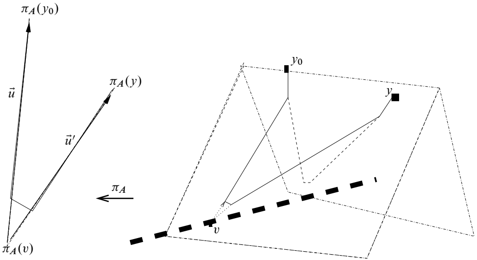
Figure 3: The loop that prevents blocking. Filled boxes represent b vertices. The left hand is the \pi_A projection image of the loop on the right.
