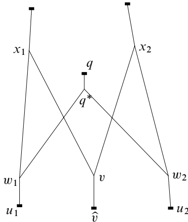
Figure 2: The loop in the proof of Proposition 4.4.4. Filled boxes are H_{\ell'} vertices.
