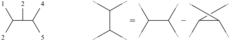
Figure 1. A tree in \mathcal{T}(5) , and an IHX relation
