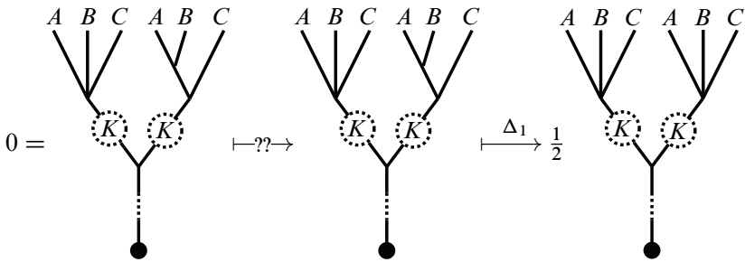
Figure 5. The tree, J , in the middle has a type (4) \text{Hall}_1 problem, since the expanded tree on the left is equal to zero in \mathbb{Z}[\frac{1}{2}] \otimes \mathbb{L}_0 . The image of J under \Delta_1 is pictured on the right. (The sub-trees indicated by the dotted arcs are all trivalent.)
