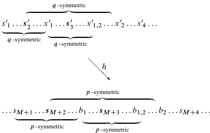
Figure 5: The configuration of symmetric arcs
