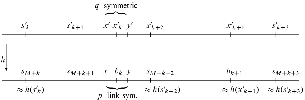
Figure 6: The relative point in the induction step. Here \approx stands for “belongs to the same arc component in the same link”.
