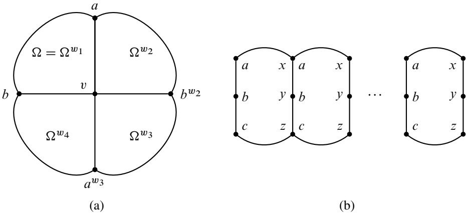
Figure 5: Proof of Theorem 1.12. (a) Cycles packed around a vertex. Note that w_2 \in \langle a \rangle w_1 = \langle a \rangle , w_3 \in \langle b \rangle w_2 , w_4 \in \langle a \rangle w_3 , and so forth. (b) A linear cellulation of a disk in C_n^e .
