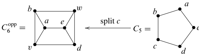
Figure 3: C_6^{\text{opp}} and C_5
