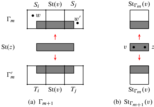
Figure 1: Proof of Lemma 3.5(6)
