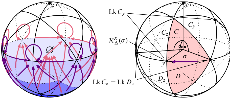
Figure 4: The (\Delta, x) -restriction in an apartment of \text{Flag}(\mathbb{P}_3(F)) containing x . (Here x is the midpoint of an edge joining a point and a hyperplane of \mathbb{P}_3(F) .)
