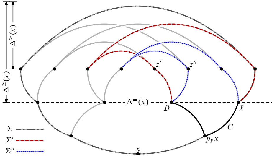
Figure 7: The construction of antipodes in \Delta^>(x)
