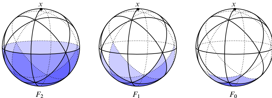
Figure 5: The filtration of an apartment of \text{Flag}(\mathbb{P}_3(F)) containing x . (Here x is the midpoint of an edge joining a point and a hyperplane of \mathbb{P}_3(F) .)
