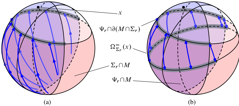
Figure 2: Via geodesic projection with center x we get (a) a homotopy equivalence \Psi_r \cap M \approx \Psi_r \cap \partial(M \cap \Sigma_r) and (b) a homeomorphism of \Psi_r \cap \partial(M \cap \Sigma_r) and a coconvex subset of \Omega_{\Sigma_r}^-(x)
