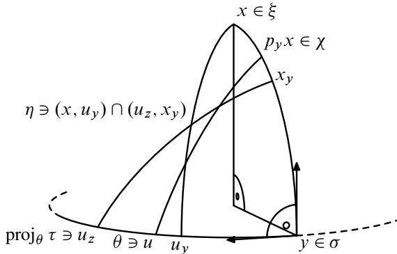
Figure 6: d(u_z, x) = \pi/2 implies \text{proj}_{\theta \cup \chi} \xi = \eta = \text{proj}_{\theta \cup \chi} \text{proj}_\theta \tau
