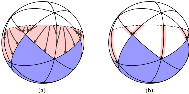
Figure 1: Deformation of a coconvex support onto the supported subcomplex
