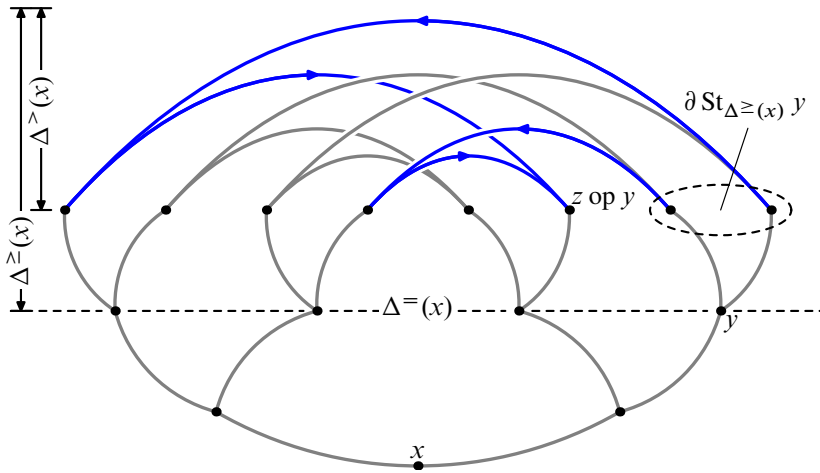
Figure 3: The segments joining \partial \text{St}_{\Delta^{\geq}(x)} y with z \text{ op } y are contained in \Delta^>(x) . Hence, the boundary of the \text{St}_{\Delta^{\geq}(x)} y is contractible in \Delta^>(x) . (Here \Delta is the flag complex of the projective plane over \mathbb{F}_2 .)
