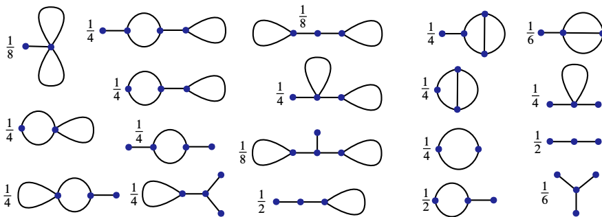
Figure 3: Diagrams with 1-vertices and 2-vertices contributing to S_3
