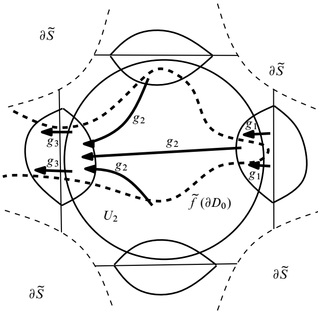
Figure 7: Illustration of the proof of Lemma 5.1
