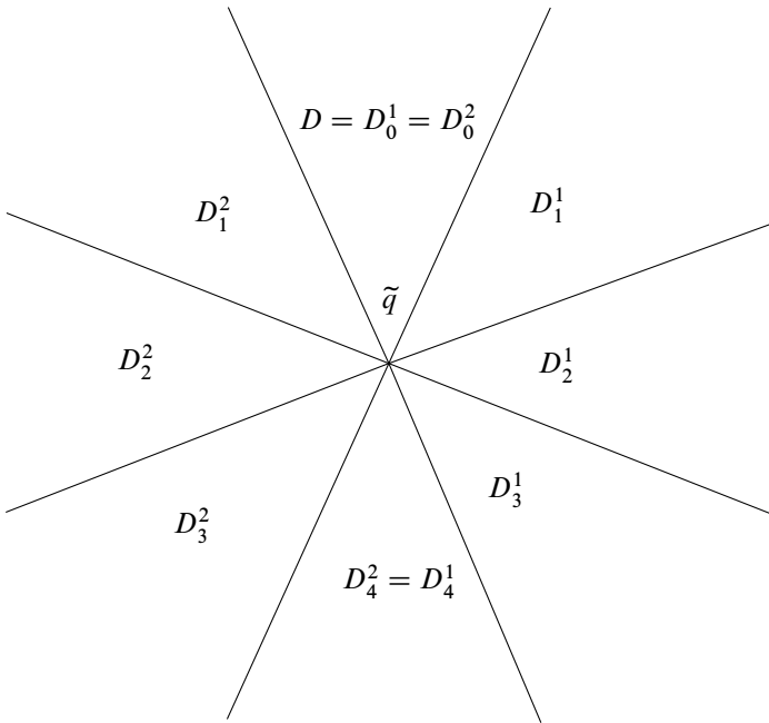
Figure 11: The D_i^j for a genus 2 surface
