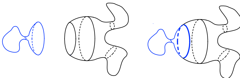
Figure 4: Combining metrics in \mathcal{Riem}_{\text{lens}(0)}^+(D^n) that have complementary boundaries (left) gives rise to a psc-metric on S^n (right)
