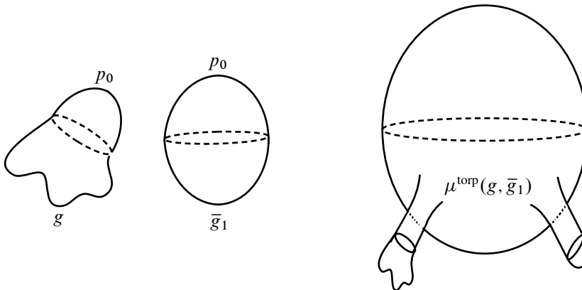
Figure 12: The metrics g, \bar{g}_1 and \mu^{\text{torp}}(g, \bar{g}_1)
