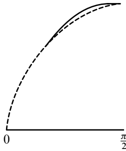
Figure 5: Comparing the graph of \eta_1 with the graph of the standard sin function represented by the dashed curve
