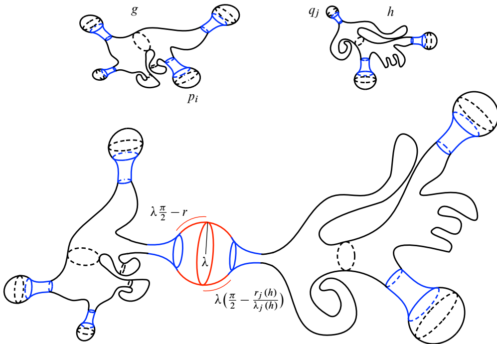
Figure 19: The metric J_{ij}^{bulb(\lambda,r)}(g, h) (bottom) obtained from g (left) and h (right)
