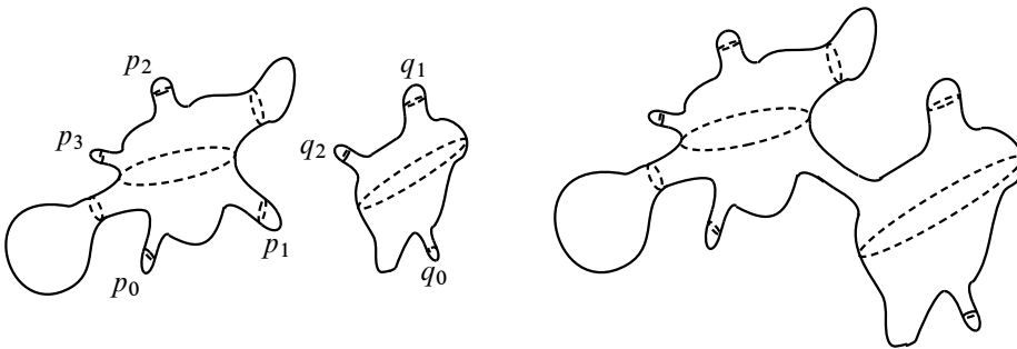
Figure 7: The metric J_{12}(g, h) (right) formed by combining g and h (left)
