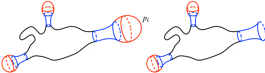
Figure 17: A metric g \in \mathcal{Riem}_{\text{bulb}(p)}^+(S^n) (left) and \text{Cut}_{p_i, \lambda_i(g)\pi - r_i(g)}(g) , the metric on D^n obtained by cutting the i^{\text{th}} head from g (right)
