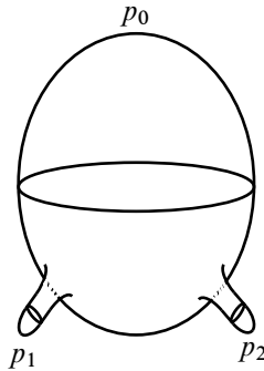
Figure 9: The metric g_3^m with three torpedo caps
