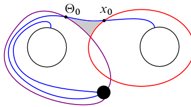
Figure 7.5: The portion of \mathcal{H}_{\alpha\delta\beta} considered in Claim 7.5
