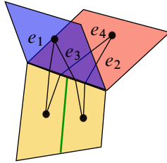
Figure 6: A switching locus
