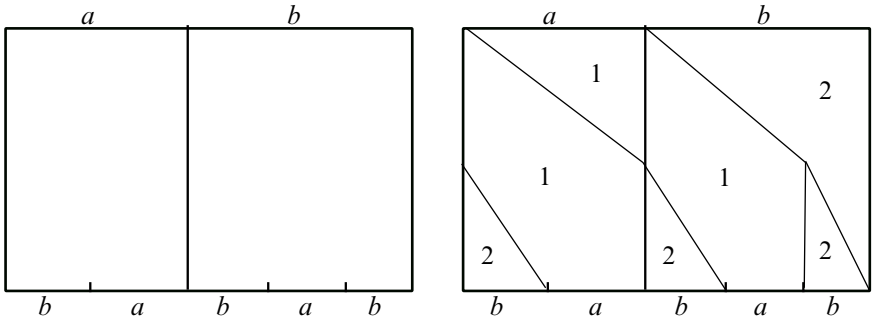
Figure 12: Mapping torus and folded mapping torus
