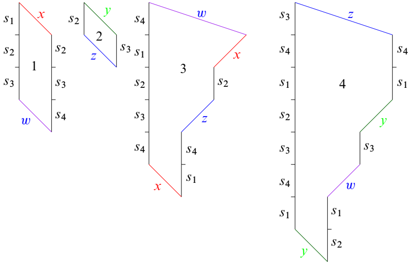
Figure 17: The discs in X
