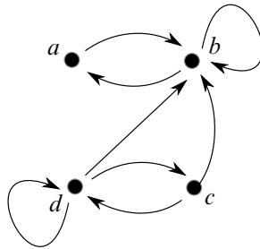
Figure 15: Digraph associated to the train-track map f
