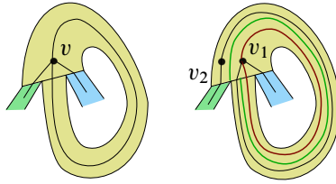
Figure 5: Vertical subdivision when digraph has a self edge
