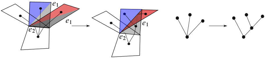
Figure 8: Effect of folding on the digraph
