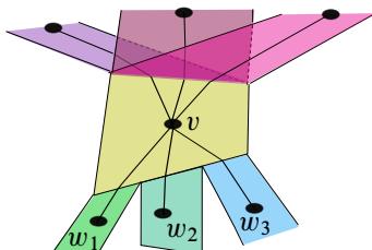
Figure 2: A section of an embedded dual digraph
