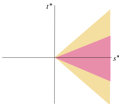
Figure 19: The McMullen cone \mathcal{T} (outer) and DKL-cone \mathcal{A}_f (inner)
