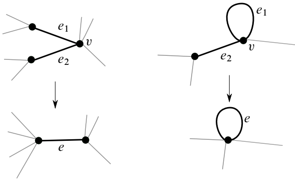
Figure 10: Two examples of folding maps
