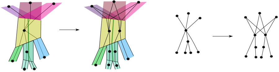
Figure 3: An allowable vertical subdivision, and effect on the directed dual digraph
