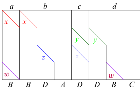
Figure 16: The complex X
