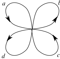
Figure 14: Four petal rose with directed edges
