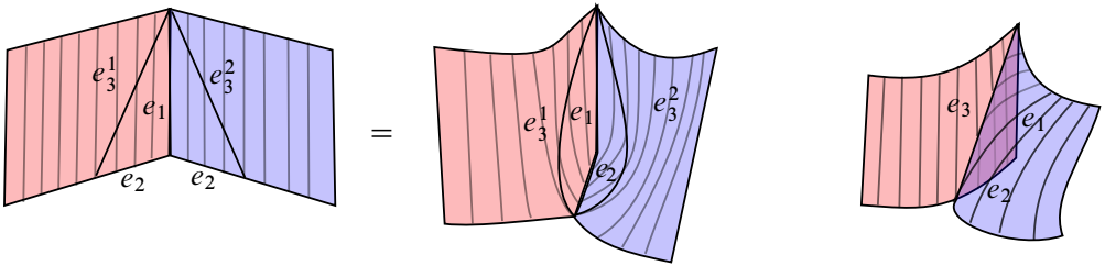
Figure 7: The left and middle diagrams depict the two 2–cells sharing the edges e_1 and e_2 ; the right diagram is the result of folding.
