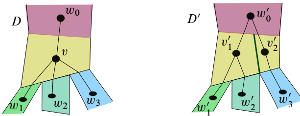
Figure 4: Vertical subdivision of one cell
