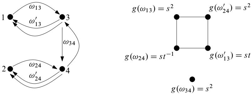
Figure 18: The dual digraph is on the left and the labeled cycle complex is on the right.
