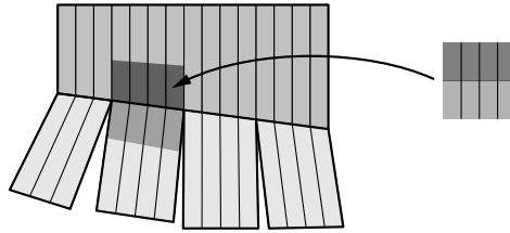
Figure 1: A hinge on a branched surface
