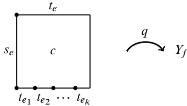
Figure 9: A cell of the mapping torus of a train-track map
