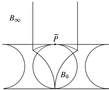
Figure 2: Le double cône \text{Cone}_0(D_0) \cap \text{Cone}_\infty(D_\infty)
