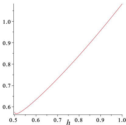
Figure 9: Graphe du majorant
