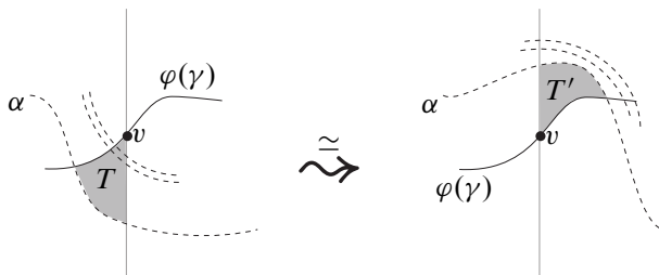
Figure 12: A shift over a vertex v
