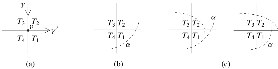
Figure 11: (a) A neighborhood of v . (b) The upward triangle T_1 . (c) As \alpha has no self-intersection, T_2 cannot be a triangular region without creating a bigon.
