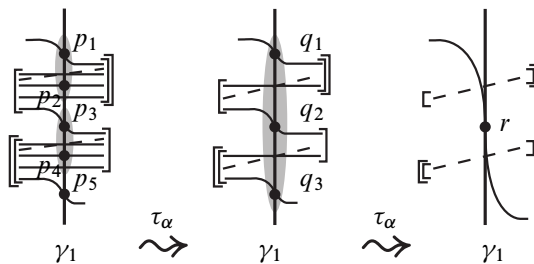
Figure 18: Equivalence classes are shaded. In the left-most configuration, we have i_\alpha(p_1) = i_\alpha(p_2) = q_1 , i_\alpha(p_3) = i_\alpha(p_4) = q_2 , and i_\alpha(p_5) = q_3 , while in the second twist i_\alpha(q_i) = r for each i .
