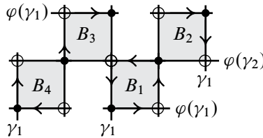
Figure 3: Various initially parallel regions in a collection \mathcal{R}(\mathcal{P}) , where we have given the arcs the orientations which induce the standard orientation on B_1 . Region B_1 has the opposite orientation of B_2 and B_3 (so B_2 and B_3 have the same orientation), while the given orientations do not orient B_4 .
