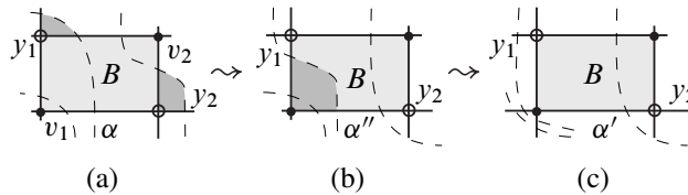
Figure 27: Shift-isotoping \alpha so that B is the prescribed pre-image
