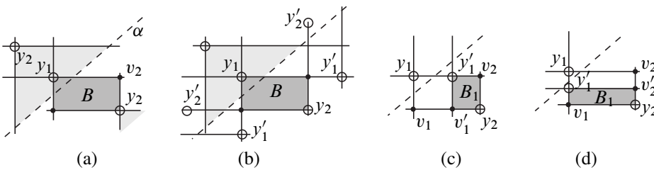
Figure 26: Figures for Lemma 3.29, case (2)
