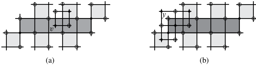
Figure 41: Figures for Lemma 4.18. The region B^c is darkly shaded, the basic regions of B lightly.
