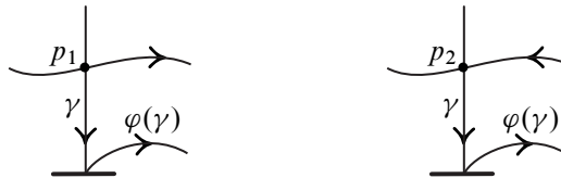
Figure 1: p_1 is a positive, p_2 a negative, point of \gamma \cap \varphi(\gamma) . This figure introduces the conventions, to be followed throughout the paper, that elements of a given arc collection \Gamma are drawn as straight lines, their images under some diffeomorphism curved, while in any figure with multiple line weights, the thickest is reserved for the boundary of \Sigma .
