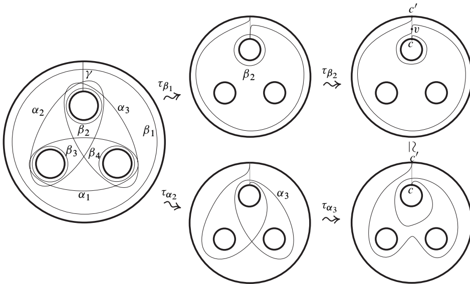
Figure 7: On the left are the curves of the well-known lantern relation on \Sigma_{0,4} . Setting \omega_1 = \tau_{\beta_4} \tau_{\beta_3} \tau_{\beta_2} \tau_{\beta_1} , \omega_2 = \tau_{\alpha_3} \tau_{\alpha_2} \tau_{\alpha_1} , the lantern relation tells us that \omega_1, \omega_2 are factorizations of a common \varphi \in \text{MCG}(\Sigma) . Clearly, for the arc \gamma indicated, the intersection point v \in \varphi(\gamma) \cap \gamma in the upper right figure is fixable under \omega_1 . However, as is clear from the lower sequence of figures, v is not fixable under the factorization \omega_2 . Thus the right position \mathcal{P}_{\omega_1} contains the point v as well as the endpoints of \gamma , while \mathcal{P}_{\omega_2} contains only the endpoints of \gamma .
