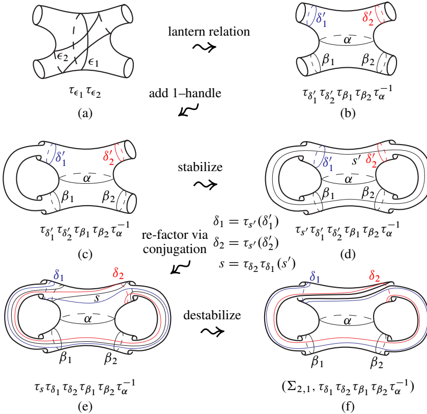
Figure 45: (\#^2(S^1 \times S^2), \xi_{s'}) is supported by (\Sigma_{2,1}, \tau_{\delta_1} \tau_{\delta_2} \tau_{\beta_1} \tau_{\beta_2} \tau_{\alpha}^{-1})
