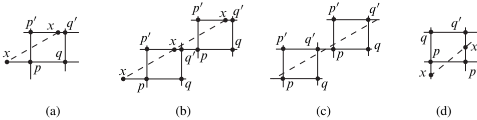
Figure 23: Figures for Lemma 3.25
