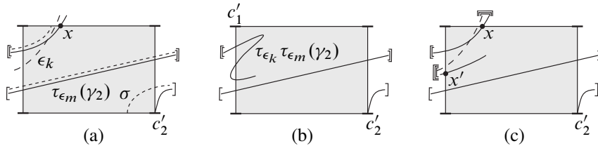
Figure 55: The neighborhood A of \epsilon_m , and the various arcs it intersects. Dark vertical lines are now segments of \gamma_2 .
