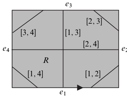
Figure 32: Representatives of each possible type of arc on R
