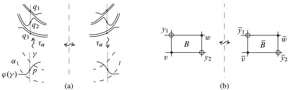
Figure 20: (a) A point p \in \gamma \cap \varphi(\gamma) , its image set i_{[\alpha]}(p) , and the reflections of each of these (note that the dots here are simply for labeling purposes, and not meant to indicate \bullet -points). (b) Reflecting a region.
