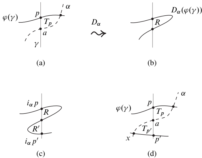
Figure 15: (a) An upward point, and (b) a corresponding bigon in the image. (c) Canceling bigons, and (d) corresponding paired regions.
