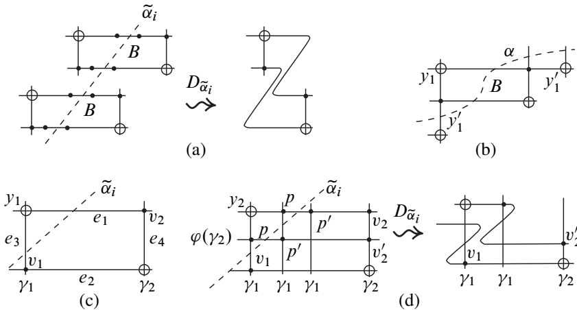
Figure 24: (a): A vertical intersection and the effect of the corresponding D_{\tilde{\alpha}_i} on the lifted region. (b) If a vertical segment of \alpha \cap B is contained in an upward triangle, then B cannot be a pre-image. (c) A corner intersection, and (d) the effect of D_{\tilde{\alpha}_i} .
