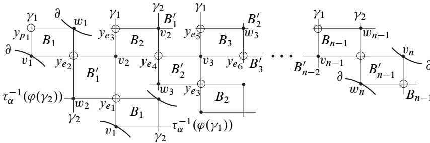
Figure 37: A schematic overview of the position \mathcal{P}^* constructed in Lemma 4.12. The picture is of the universal cover of \Sigma , along a lift of \tau_\alpha^{-1}(\varphi(\gamma_1)) . As usual, all lifts of an object are given the same label as the original object.
