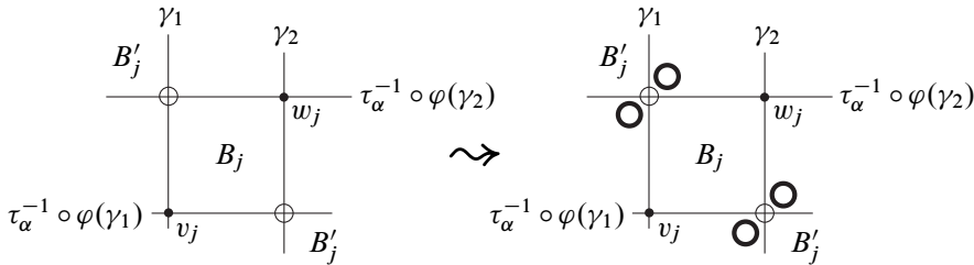
Figure 43: Modification \Sigma^{j-1} \rightsquigarrow \Sigma^j . The thick circles indicate boundary components introduced by the modification.
