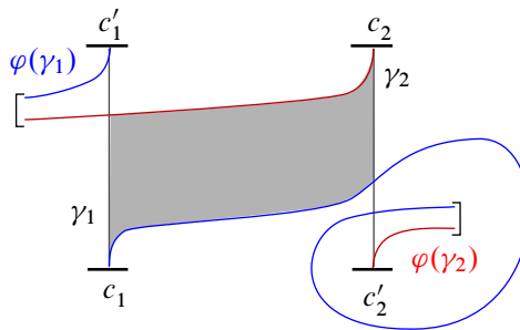
Figure 5: The augmented open book decomposition (\Sigma, \varphi, \{\gamma_1, \gamma_2\}) does not admit a consistent right position. The pair of brackets is meant to signify an identification, ie what goes in one comes out the other. This convention is followed throughout the paper.
