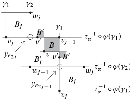
Figure 42: Figure for Lemma 4.19.
