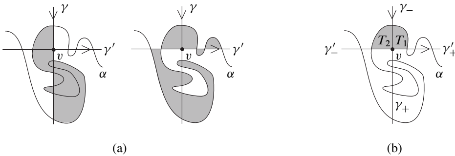
Figure 10: (a) The shaded regions are distinct maximal bigon chains. (b) As each chain from (a) has a vertex in each of the triangular regions T_1, T_2 , the bigon collection \mathcal{B}_{T_1} = \mathcal{B}_{T_2} includes each intersection point of each chain. In this example, \sigma_v(\mathcal{B}_{T_1}) = (0, 1, 1, 0) , so the collection is downward. Note that T_1 is an essential downward triangular region (Definition 3.11), while T_2 is non-essential.
