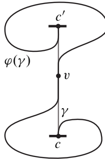
Figure 2: \mathcal{P} = \{c, v, c'\} is a right position of (\Sigma, \varphi, \{\gamma\}) . There are three distinct horizontal segments: h_{c,v} , h_{v,c'} , and h_{c,c'} .
