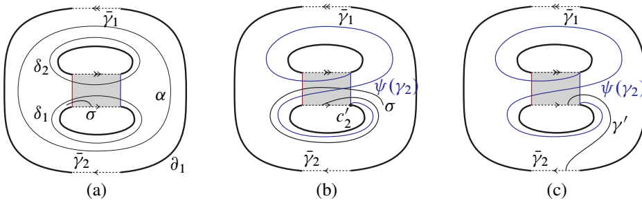
Figure 50: Arcs of \epsilon \cap \Sigma'
