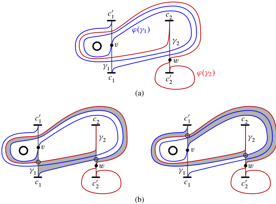
Figure 4: (a): The triple (\Sigma, \varphi, \{\gamma_1, \gamma_2\}) admits a consistent right position. The pairs of completing discs are shaded in (b).
