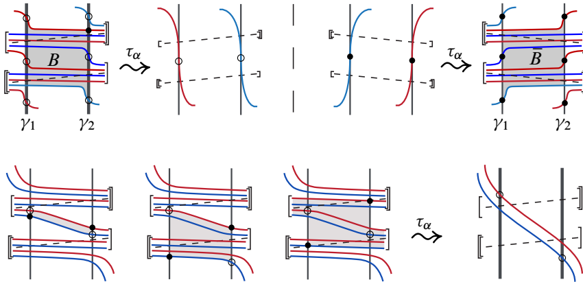
Figure 21: Above: To the left, a collapsed region B , and its (trivial) image. To the right, the reflection of B is a created region \bar{B} . Below: The three figures to the left are various regions in a common configuration, which is mapped by \tau_\alpha to the right-most figure. From left to right, these 3 regions are non-collapsed (satisfies condition (1) but not condition (2)), non-collapsed (satisfies condition (2) but not condition (1)), and collapsed (but not embedded).
