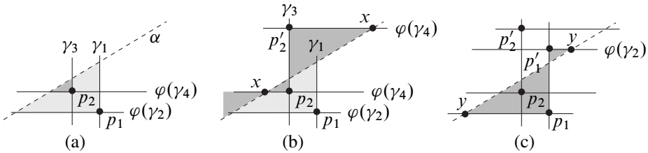
Figure 17: (a) Region T_{p_1} is lightly shaded, T_{p_2} is dark. (b) The pair of regions T_{p_2} and T_{p'_2} are darkly shaded. As usual, the figures are in the universal cover, with all lifts of a given object given the same label as the object. (c) The region pair T_{p_1} and T_{p'_1} is shaded.
