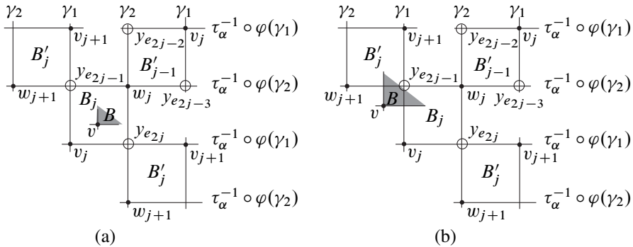
Figure 44: The setup for the argument of Lemma 4.20. As usual, the figure illustrates the situation in the universal cover of the surface; lifts of a common object are labeled identically.
