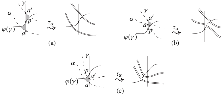
Figure 14: The point p is downward in 2 distinct triangles. (a), (b), and (c) show representatives of the possible shift-isotopy classes, each of which gives a distinct point i_\alpha(p) , while i_{[\alpha]}(p) is the same for each.
