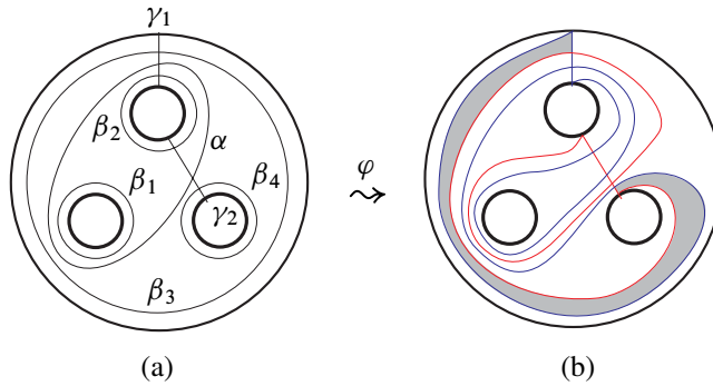
Figure 6: (a) Surface and curves for the open book decomposition denoted (\Sigma_{0,4}, \tau_\alpha^{-2} \tau_{\beta_1}^n \tau_{\beta_2}^{n_2} \tau_{\beta_3} \tau_{\beta_4}) . (b) The triple (\Sigma, \varphi, \{\gamma_1, \gamma_2\}) does not admit any consistent right position, but \varphi is right-veering for all m, n \geq 1 .
