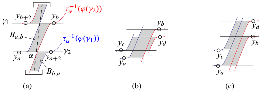
Figure 39: (a) The region B_{a,b} corresponding to the path \eta_{a,b} , and complementary B_{b,a} corresponding to \eta_{b,a} . The curve \alpha is the dashed line. (b) Nested, and (c) non-nested regions.
