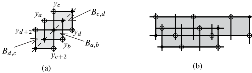
Figure 40: (a) If a basic region is non-nested, so is its complementary region. (b) Two collapsed, non-nested regions of length 1. Each is either non-empty, or has non-isolated \circ -points.
