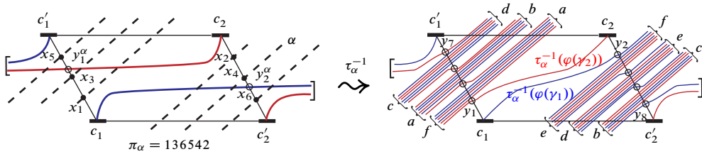
Figure 36: Above left, the various points of \alpha \cap \gamma_i and \alpha \cap \varphi(\gamma_i) . Above right, the inverse image \tau_\alpha^{-1}(\varphi(\gamma_i)) , for \alpha with \pi_\alpha = 136542 (strands terminating in brackets with like letters are meant to be identified).
