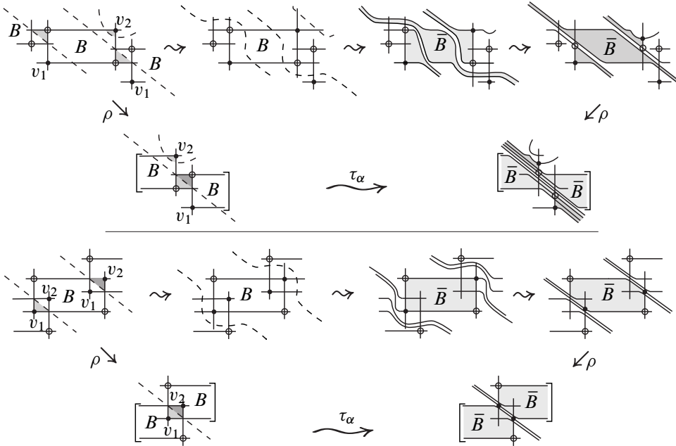
Figure 28: Examples of the steps outlined in Lemma 3.30. In each of the two figures, the lower left illustration is of some collection of triangular regions in \Sigma whose shifts cannot be done simultaneously, while each upper row is in the universal cover, and the squiggly arrows refer to, from left to right, the isotopy (\rho^{-1}\alpha) \rightsquigarrow (\rho^{-1}\alpha)' , the map D_{h_i} \tilde{\tau}_{(\rho^{-1}\alpha)} applied to the \rho^{-1}(\varphi(\gamma_j)) , and finally the isotopy of these images back to the \rho^{-1}(\tau_\alpha(\varphi(\gamma_j))) .
