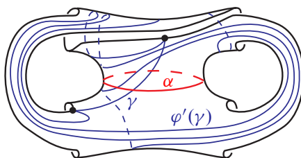
Figure 57: The arc \gamma , and its image \varphi'(\gamma) .
