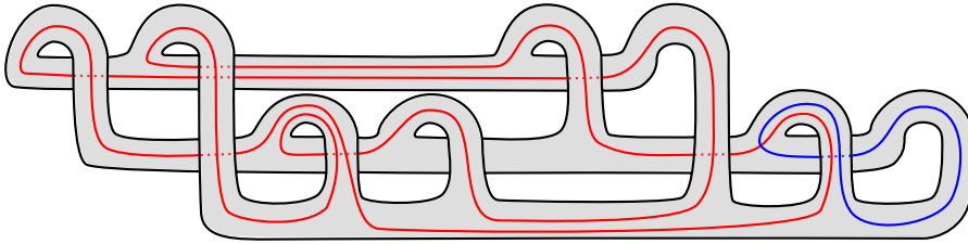
Figure 1: A quasipositive Seifert surface S (gray) for the knot 12n750 (black) containing two simple closed curves \alpha (red, left) and \beta (blue, right) such that a neighborhood of \alpha \cup \beta bounds a knot L with trivial Alexander polynomial.
