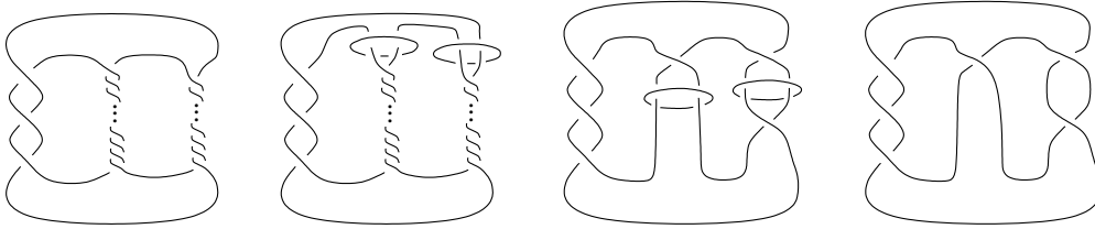
Figure 7: Examples of diagrams for K (far left), L (middle left), L_2 (middle right) and K_2 (far right) (figure from [20])
