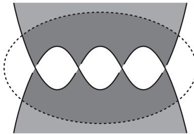
Figure 4: The subsurface of a checkerboard surface associated with a twist region
