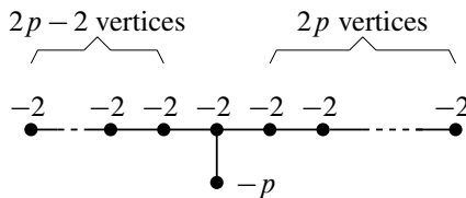
Figure 4: The plumbing graph for -Y_p
