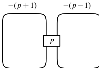
Figure 1: The manifold Y_p presented as surgery on a two-component torus link. The box indicates p positive full twists.
