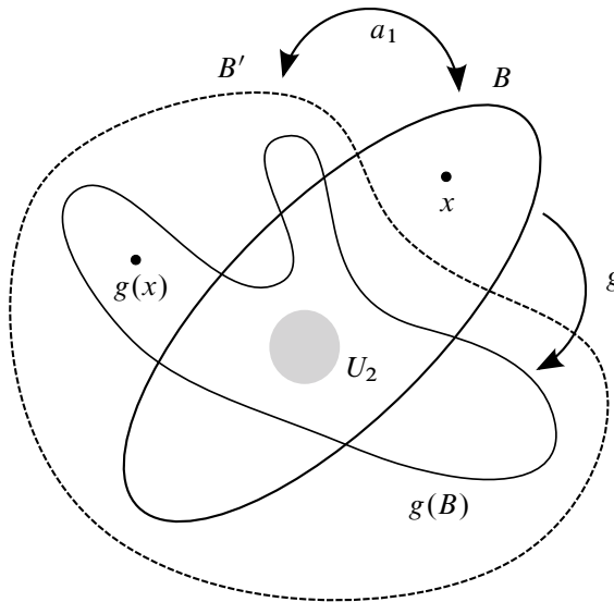
Figure 1: The balls B, g(B), and B'
