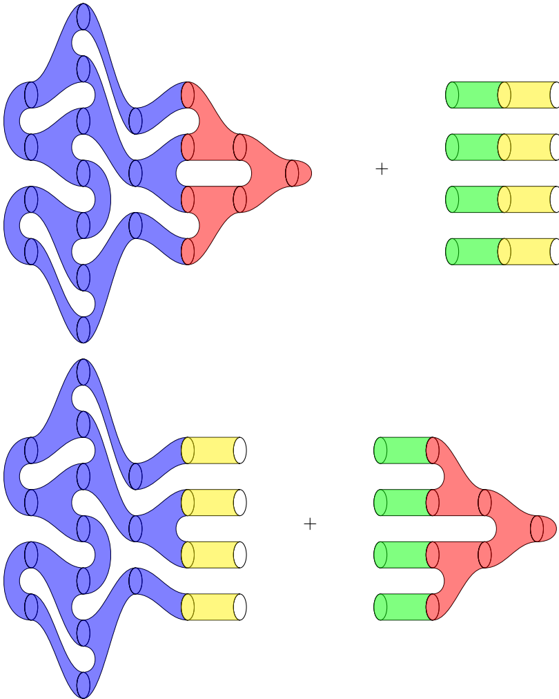
Figure 6: A picture of the relative index theorem. The operator is invertible on the parts which are not blue. The index of the operator associated to the upper picture is the index of its left part \tilde{W} . The index is preserved under cut-and-paste as indicated. The index of the operator associated to the lower picture is again the index of the left part \tilde{W} .
