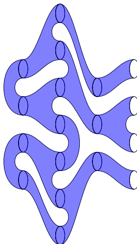
Figure 3: A picture of S^1 \times W
