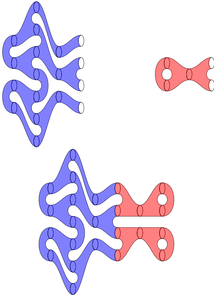
Figure 2: Pictures of W , W' and \frac{1}{2}\tilde{W} with l = 4 and l' = 2
