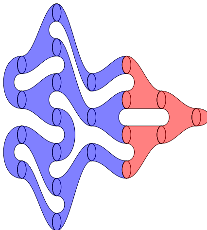
Figure 5: A picture of \tilde{W}
