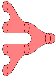
Figure 4: A picture of S^2_4 \times M
