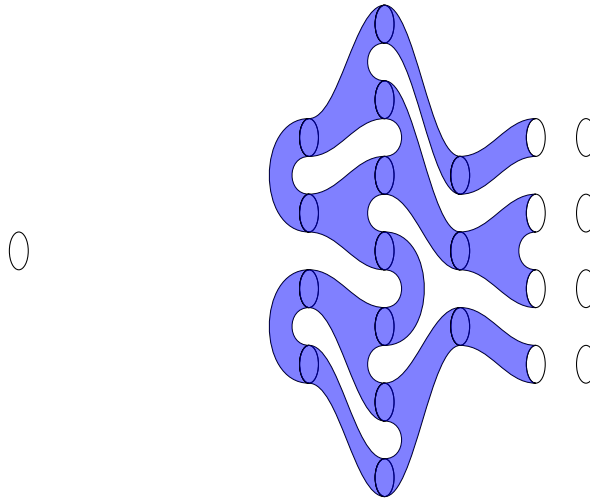
Figure 1: A picture of M and the zero bordism W of 4M
