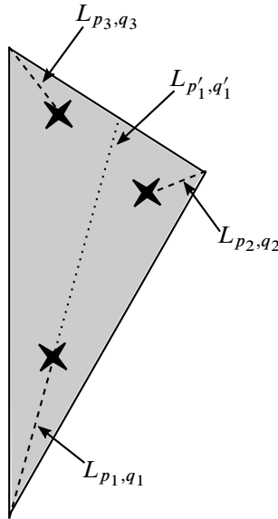
Figure 3: An almost toric picture of \mathbb{C}\mathbb{P}^2 as a smoothing of a weighted projective space \mathbb{C}\mathbb{P}(p_1^2, p_2^2, p_3^2) ; there are three singular fibres, marked by stars, with three (dashed) branch cuts. The Lagrangian pinwheels L_{p_i, q_i} live over the branch cuts. The Lagrangian pinwheel L_{p'_1, q'_1} is also depicted, living over the dotted line which is the continuation of one of the branch cuts. It intersects L_{p_1, q_1} once transversely.
