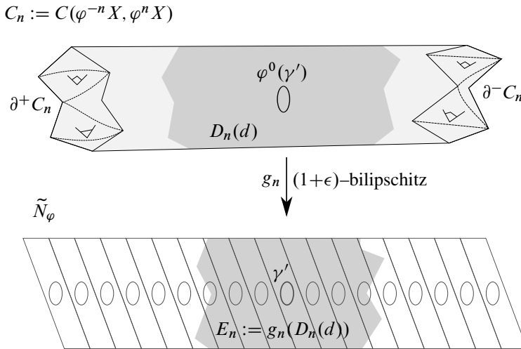
Figure 2: The map from the deep part to the infinite cyclic cover, which is shown tessellated by \varphi -translates of a fundamental domain (depicted as parallelograms), each containing a closed geodesic \varphi^k(\gamma') .
