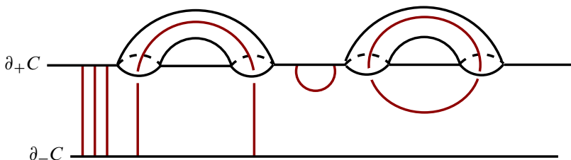
Figure 1: A vp-compressionbody (C, T) . From left to right we have three vertical arcs, one ghost arc, one bridge arc and one core loop in T . This figure was reappropriated from [36].
