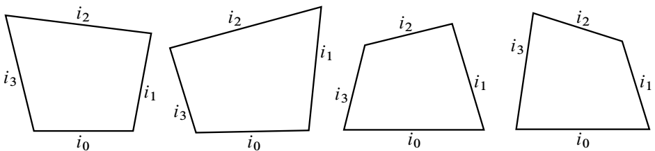
Figure 5: The four shapes of generic quadrilaterals
