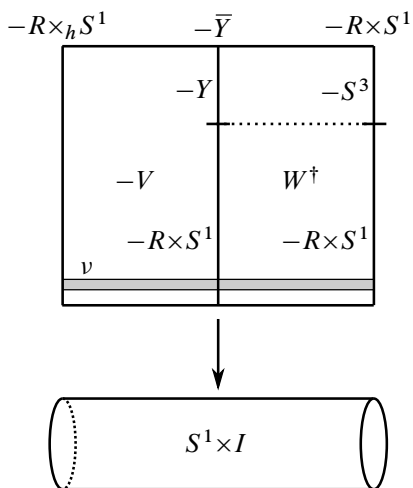
Figure 2: The composition X^\circ = -V \cup_{-\bar{Y}} W^\dagger and its Lefschetz fibration over S^1 \times [0, 1] . The region of W^\dagger above the dotted line consists of the handles coming from the given Lefschetz fibration on the Stein filling W ; the region below is just a product. The cylindrical cobordism \nu is represented in gray.
