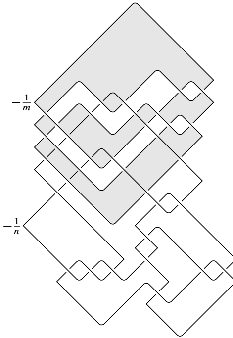
Figure 6: A hyperbolic two-component link L \subset S^3 , with a Seifert surface for the \bar{8}_{21} component shaded to make the components easier to distinguish. The closed 3-manifold Y(m, n) is constructed by Dehn surgery on L with the indicated framings.
