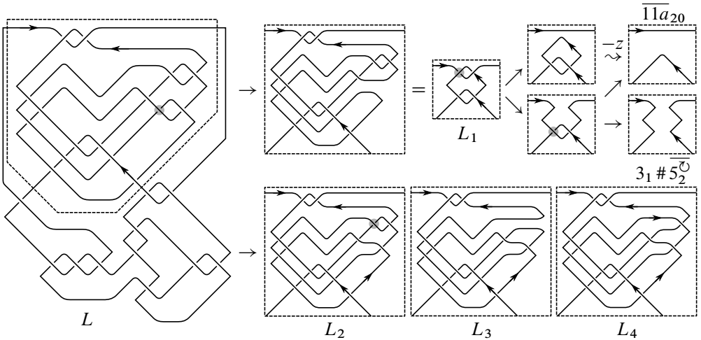
Figure 7: We compute \nabla_L(z) by applying the skein relation to L at the indicated crossings. Here the “ \overset{-z}{\rightsquigarrow} ” means that the Conway polynomial of the target is -z times that of the source, and \overline{5_2^U} denotes a \overline{5_2} knot linked with a negatively oriented meridian.
