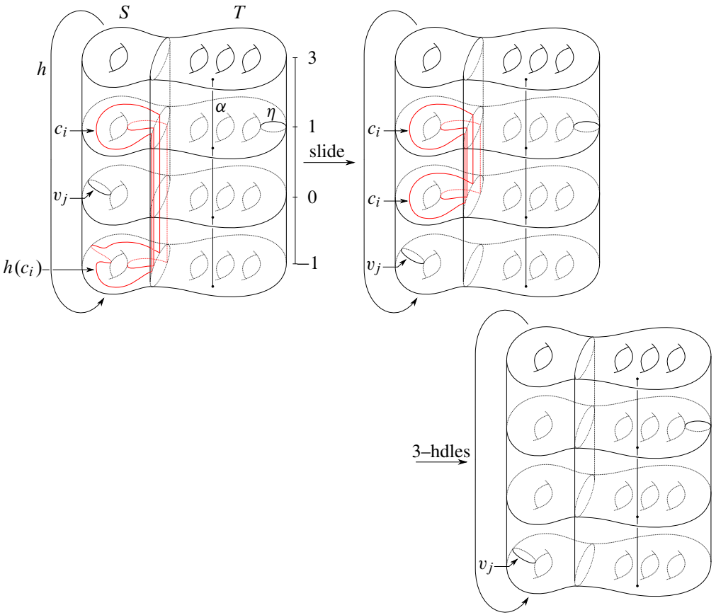
Figure 3: Left: attaching 2–handles along the \gamma_i and copies of v_j in -R \times_h S^1 ; we have labeled the top and bottom arcs of \gamma_i by c_i and h(c_i) . Center: the result of sliding the \gamma_i over the v_j handles. Right: after attaching 3–handles to cancel the \gamma_i' handles, we are left only with +1–framed attachments along the copies of v_j .
