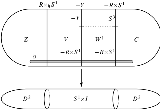
Figure 4: The Lefschetz fibration \tilde{X} = (-Z \cup -V \cup_{-\bar{Y}} W^\dagger \cup C) \rightarrow S^2
