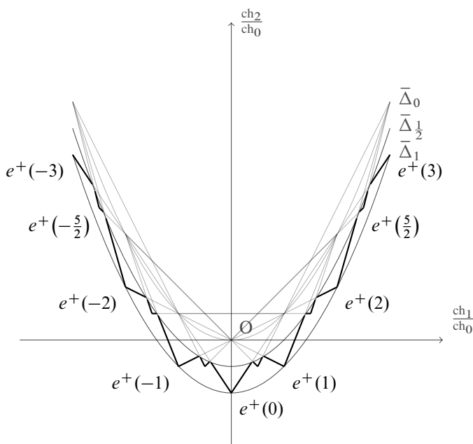
Figure 2: The Le Potier curve C_{\text{LP}}
