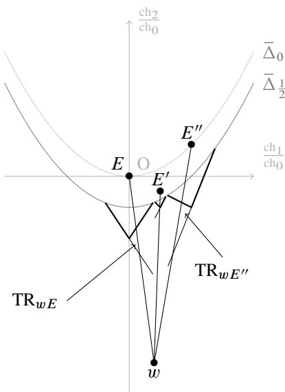
Figure 12: Definition of \text{TR}_{wE}
