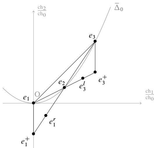
Figure 4: \text{TR}_{\mathcal{E}} and \text{MZ}_{\mathcal{E}}
