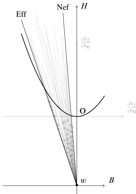
Figure 13: The stable base locus decomposition of the effective cone of \mathfrak{M}_{\mathrm{GM}}^s(4, 0, -15)
