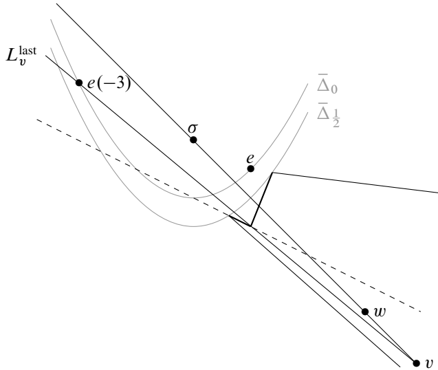
Figure 10: L_{v\sigma} is between L_{v\pm} and L_v^{\text{last}}
