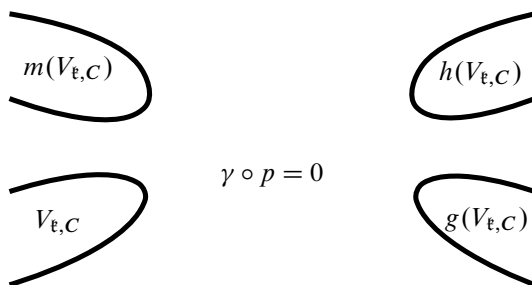
Figure 1: When \text{Stab}_\Gamma(\hat{h}) \neq A
